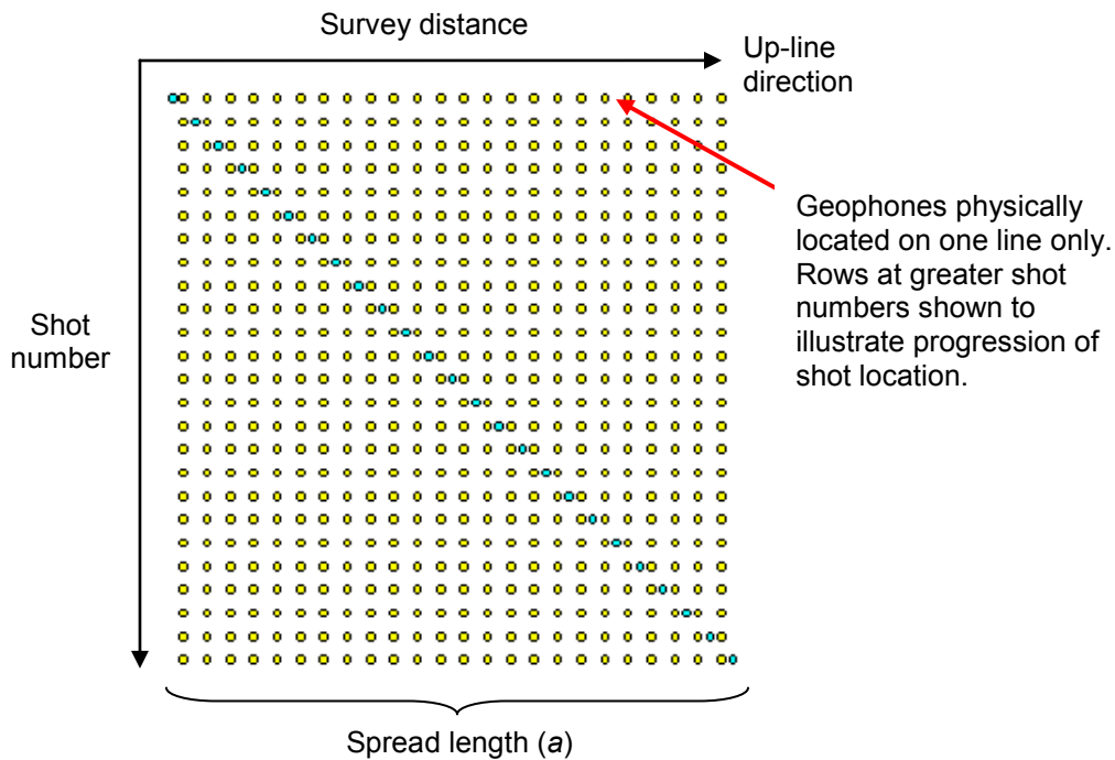
Figure 8. 2D MASW fixed receiver spread configuration.
